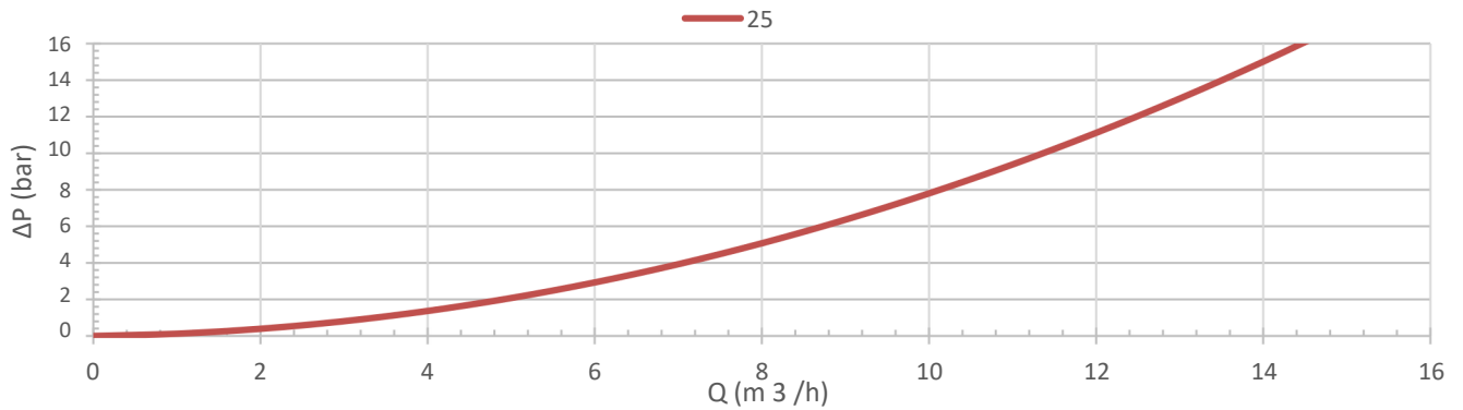
AV3FP and AV3FB 1" (DN25) AUTOMATIC PURGE
