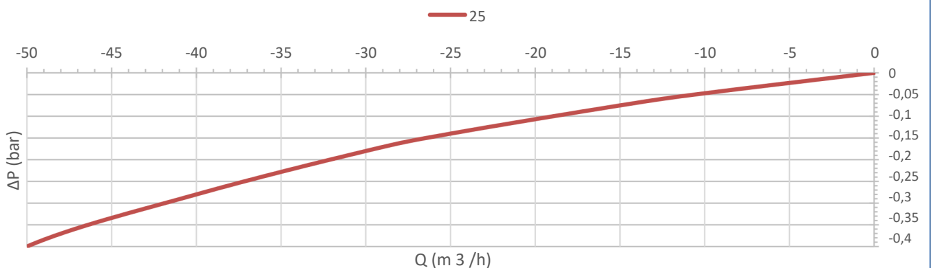
AV3FP and AV3FB 1" (DN25) KINETIC ADMISSION
