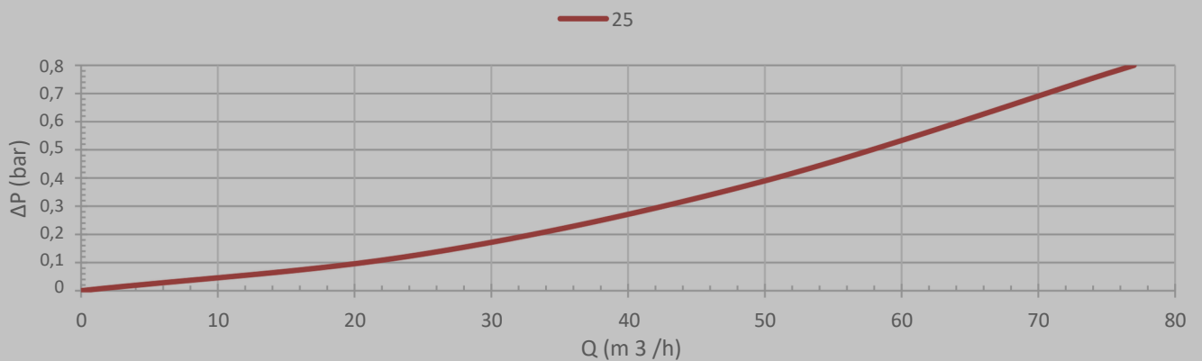
AV3FP and AV3FB 1" (DN25) KINETIC PURGE
